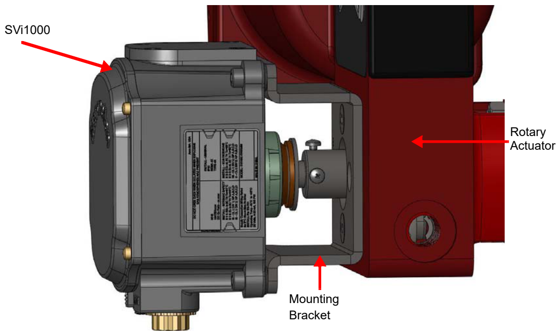
Figure 13 - Camflex with Mounting Bracket (Side View)
