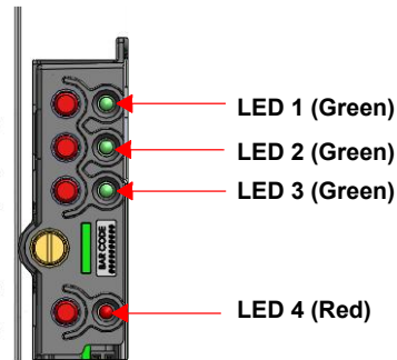
Figure 4 - SVi1000 LEDs
