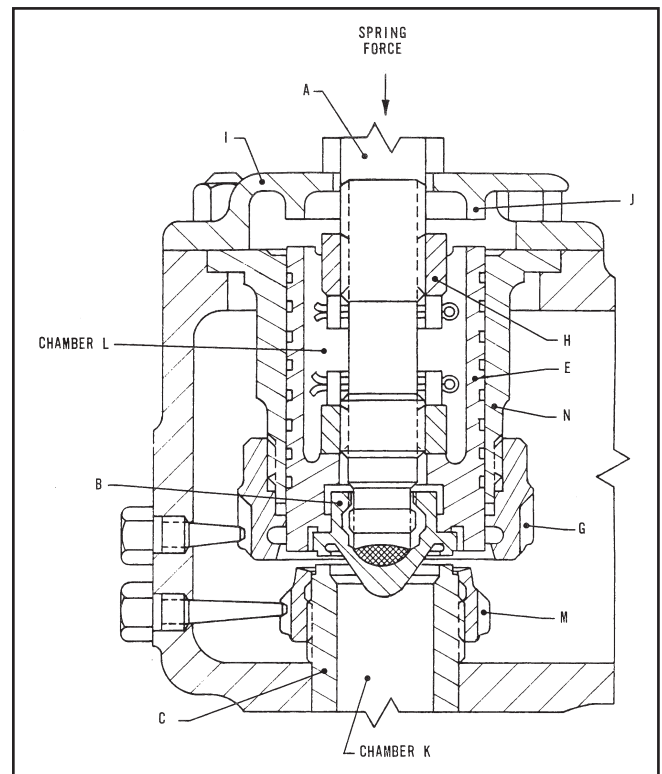
Figure 5: Valve Closing
