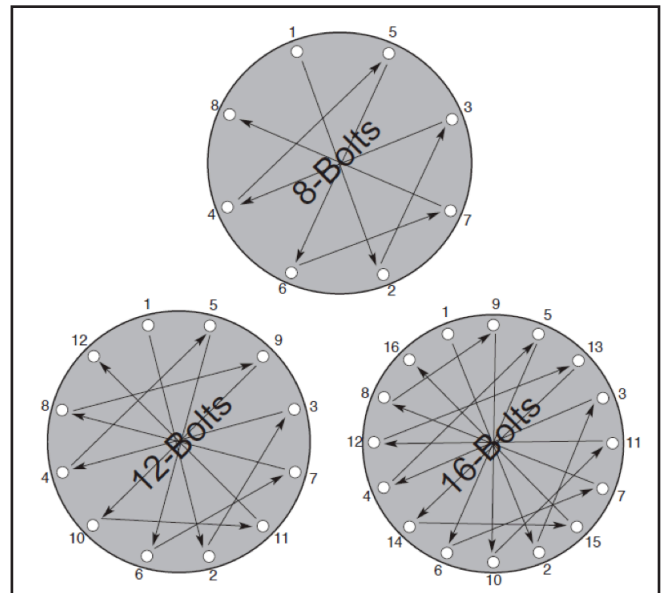
Figure 6: Torque Pattern
